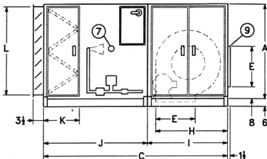
ELEVATION VIEW
